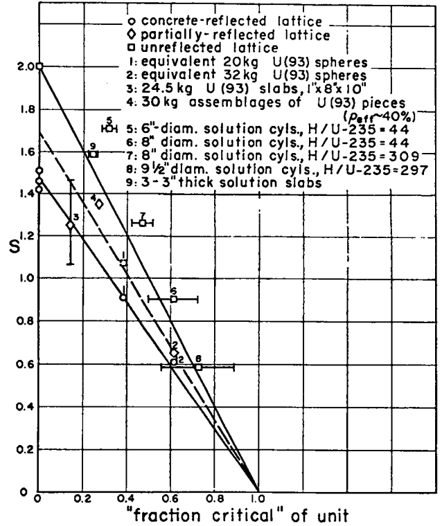
Fig. 12. Lattice-density exponent vs "fraction critical" of an isolated unit for various degrees of external reflection.
