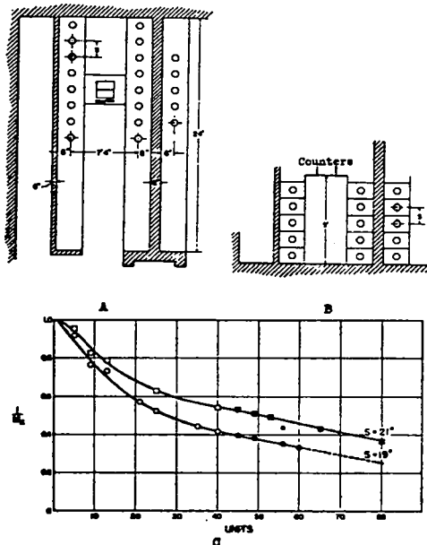
Fig. 8. Change of reciprocal cross multiplication as large capsules were positioned in a storage vault at spacings of 19 and 21 in. One side was filled before the other was started. The lonesome point, for 19-in. spacing, shows the apparent effect of four persons in the corridor.
