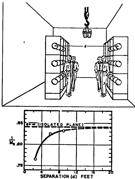
Fig. 7. Effect of separation between two planar arrays on overall cross multiplication. Each plane consisted of 12 large capsules at 30-in. spacing; neutron counters were overhead. Persons between planes did not change results.
